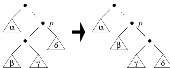
Fig. 2. Increasing the length of the rightmost path by a right rotation.
