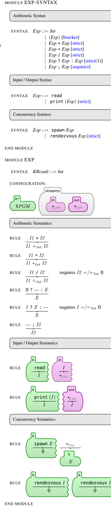
Fig. 4. \mathbb{K} definition of a calculator language with I/O (left: ASCII source; right: generated \text{\LaTeX} )
